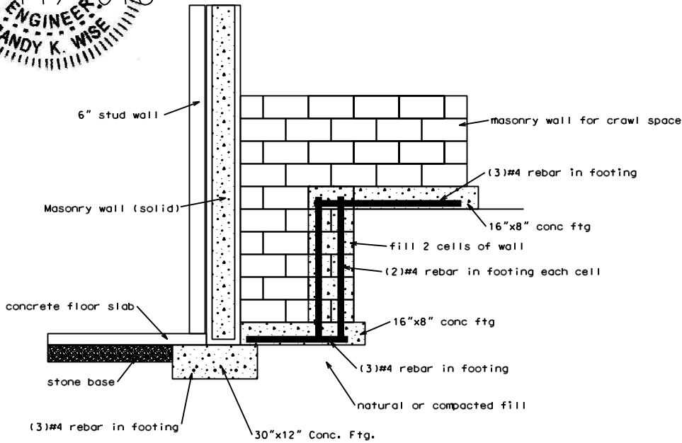
Detail for Basement/Crawl Tie-In
