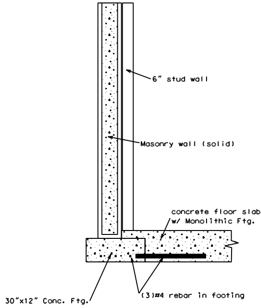
Detail for Basement/Slab Tie-In
