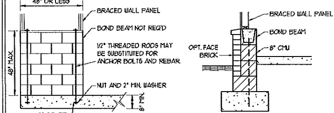
OPTIONAL STEM WALL REINFORCEMENT TYPICAL STEM WALL SECTION
