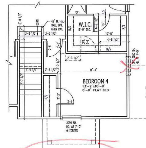
OPT. BEDROOM 4 ELEV. "A" SHOWN
