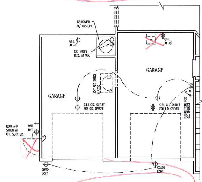
OPT. 1 CAR GARAGE
