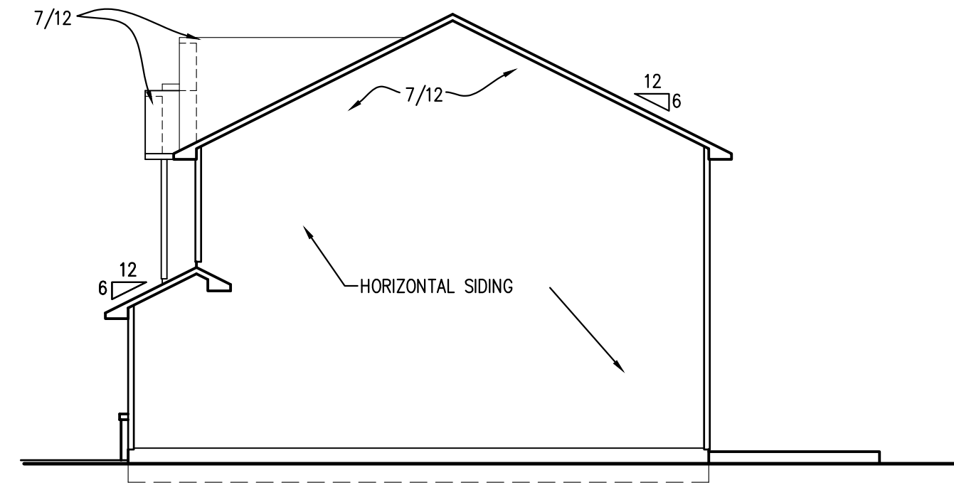
RIGHT ELEVATION 1/8" = 1'-0"
