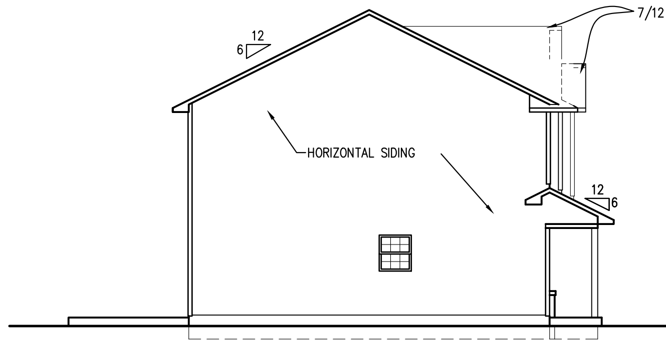
LEFT ELEVATION 1/8" = 1'-0"
