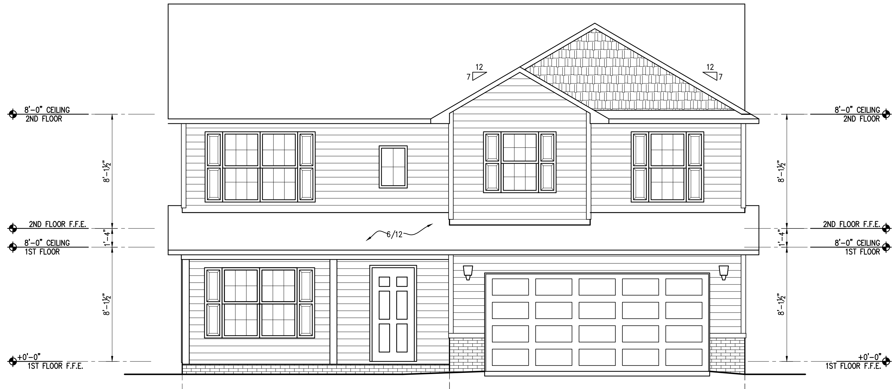
FRONT ELEVATION 1/4" = 1'-0"
