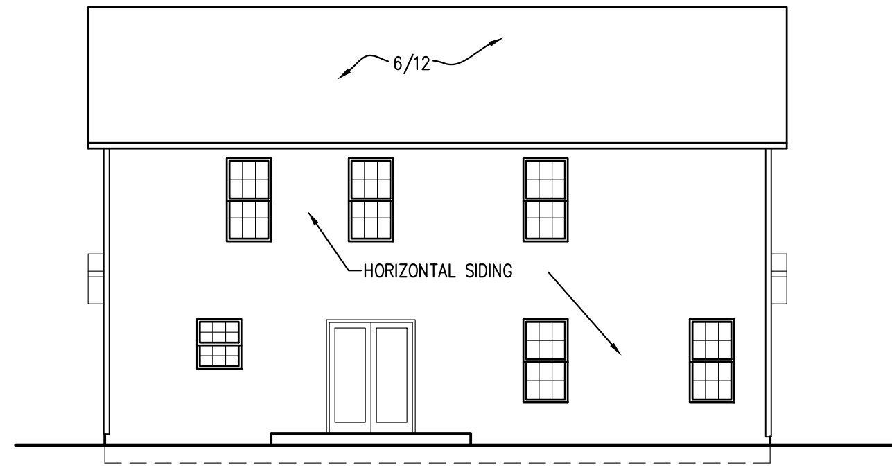
REAR ELEVATION 1/8" = 1'-0"
