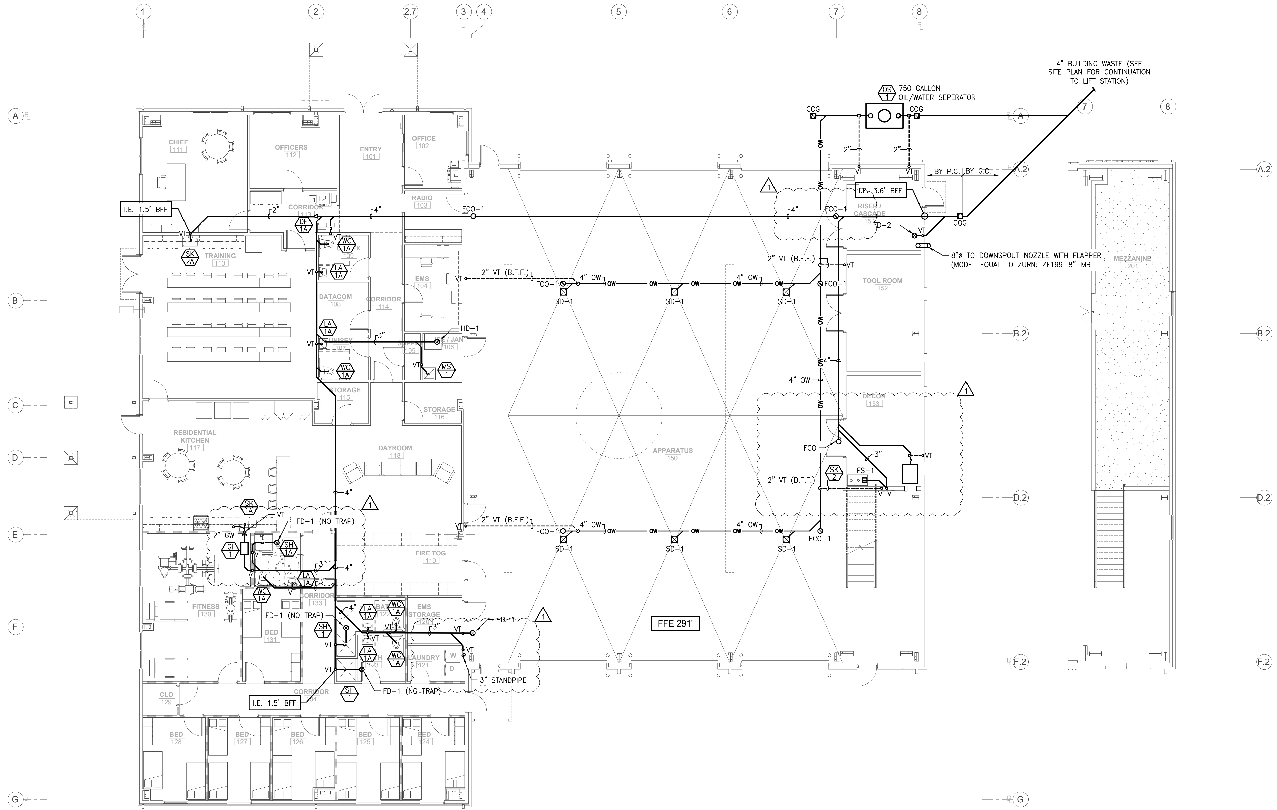
1 PLUMBING DWV PIPING PLAN SCALE: 1/8" = 1'-0"
