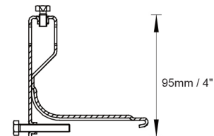
RF-12310 Hat furring channel bracket
