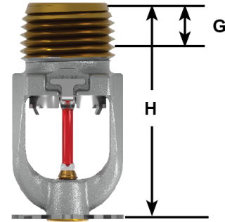
Figure – 2: Dimensions
