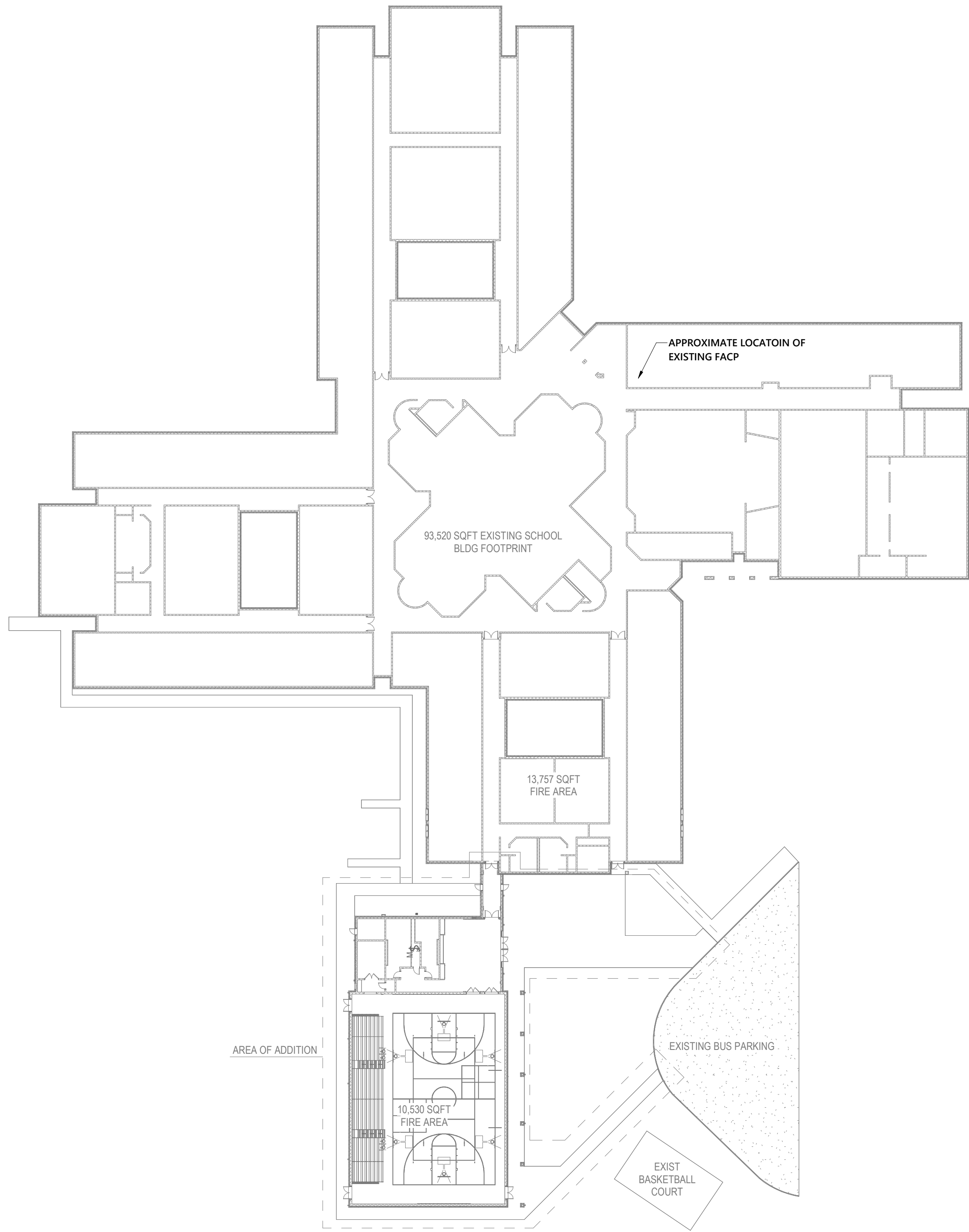
2 OVERALL FIRE ALARM PLAN 1" = 40'-0"
