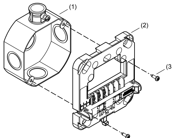
Figure 3: Mounting on a 4-in octagon electrical box
