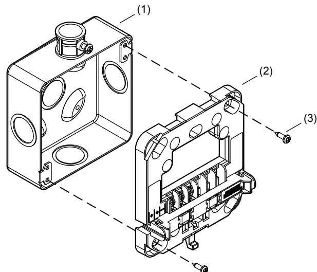
Figure 4: Mounting on a 4-in square electrical box
