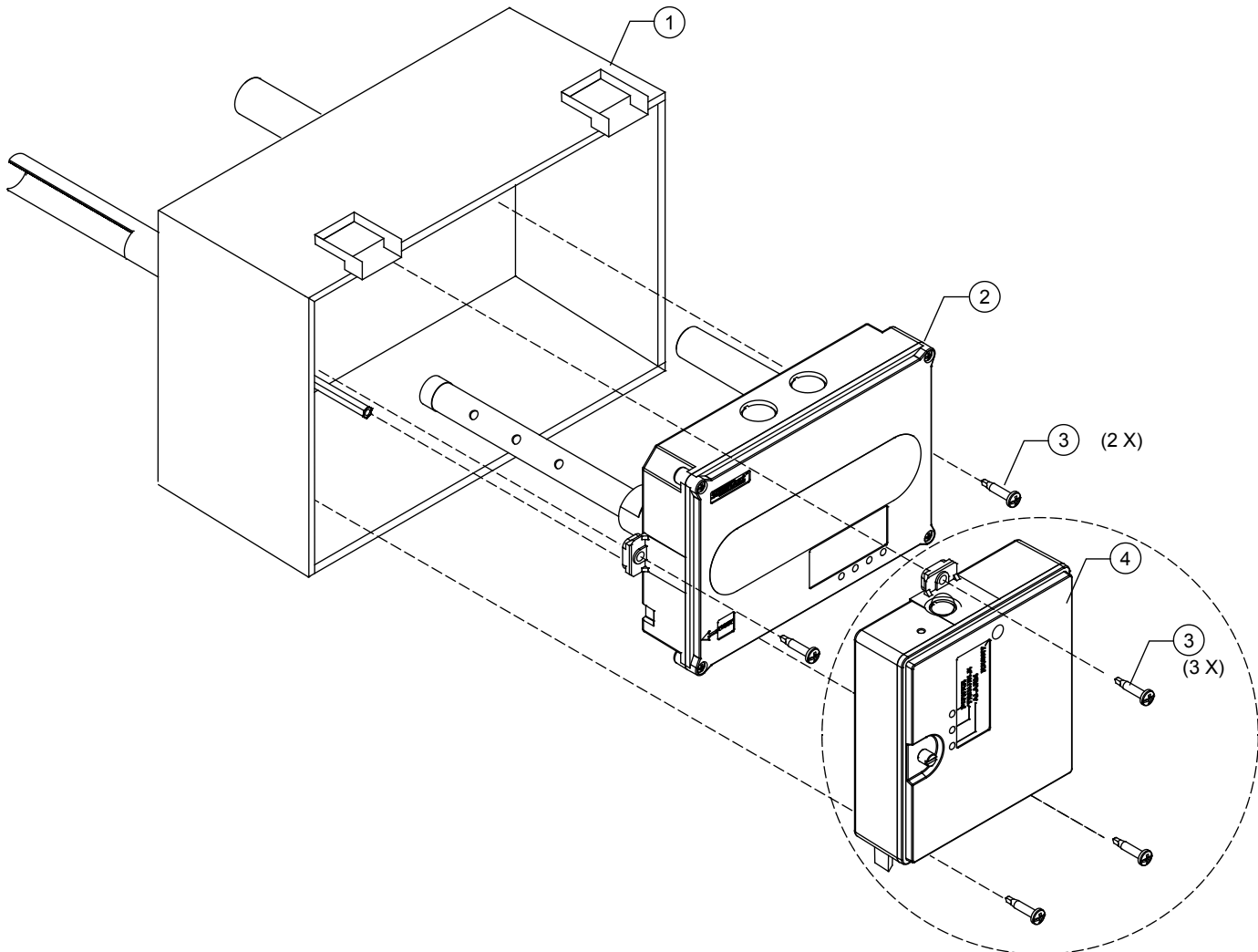
Figure 3: Mounting diagram
