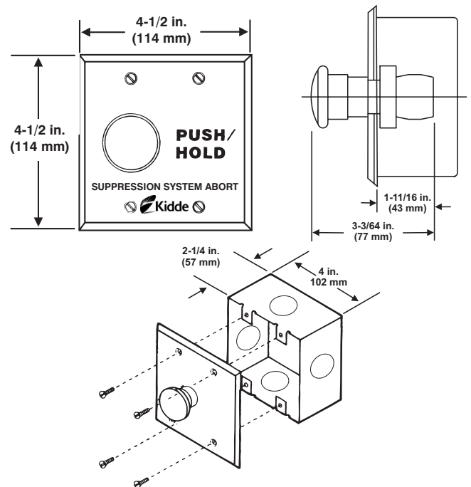
Figure 1. Dimension Details
