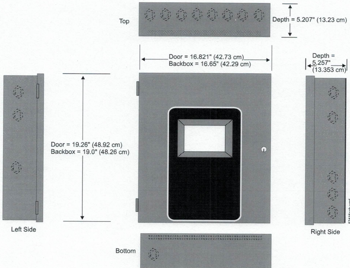
Cabinet Measurements
