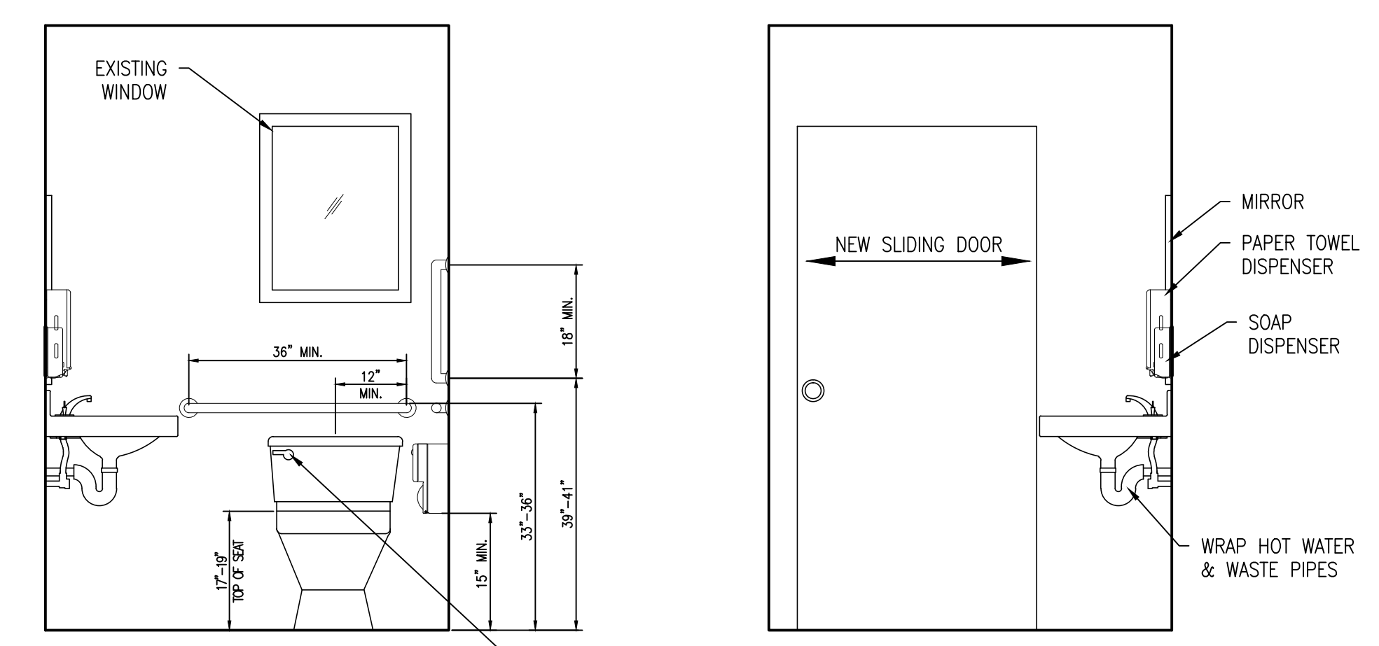
B4 ACCESSIBILITY DIMENSIONS SCALE: NTS FLUSH CONTROLS TO BE OPPOSITE THE SIDEWALL BAR
