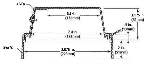
SIDE VIEW MODELS WITHOUT HORN (STI-3150 Series)
