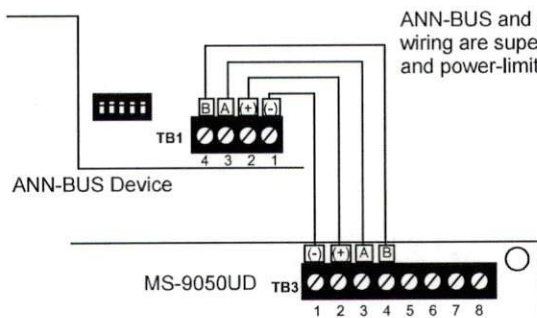
FACP Wiring to ANN-BUS Device
