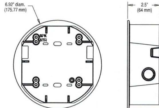
Ceiling Surface Mount Back Box
