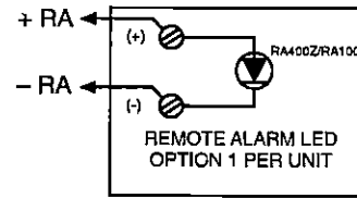
FIGURE 8. WIRING DIAGRAM FOR D355PL TO RA400Z/RA100Z:
