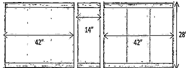
MENUBOARD DIMENSIONS
