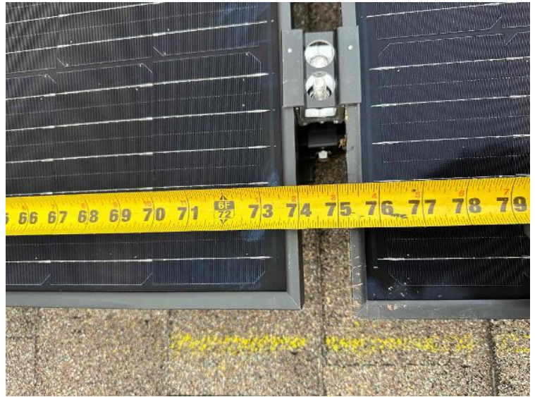
Rooftop Installation / Module Gapping: Tape Measure showing 3/8" - 1" Gap
