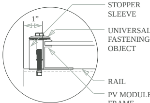
End Clamp, Front
