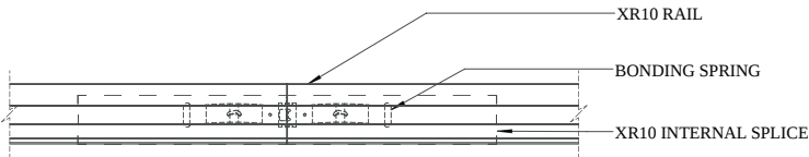
Splice Connection
