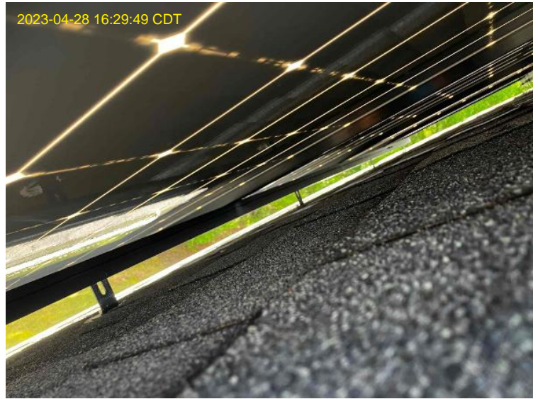
Roof/Array Work / Photo: Under Array (wire management)
