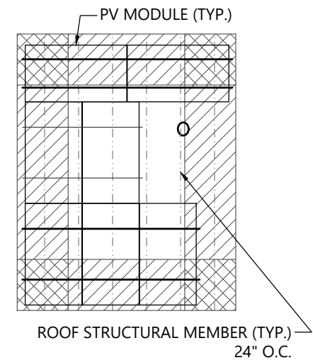
2 ROOF A ARRAY LAYOUT 1/8" = 1'-0"
