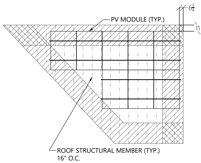
2 ROOF A ARRAY LAYOUT 1/8" = 1'-0"
