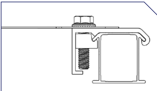
Tighten the bolt to 144 in-lbs
