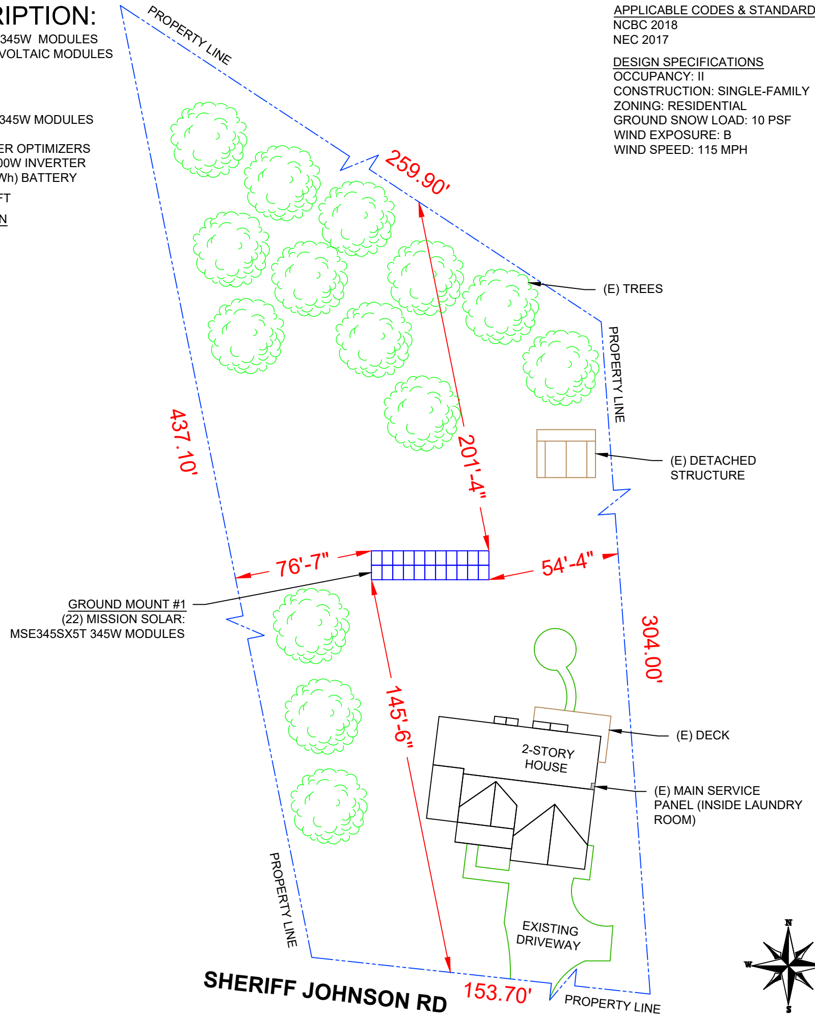
1 PLOT PLAN
