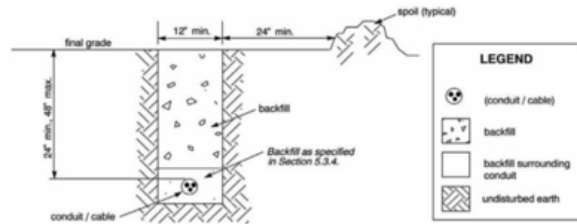
TYPICAL TRENCH DETAIL
