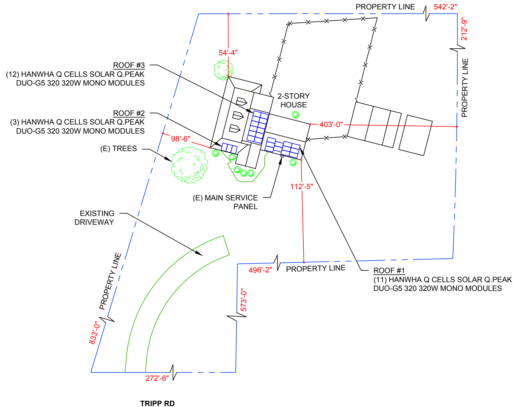
1 PLOT PLAN WITH ROOF PLAN
