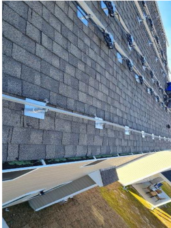
Roof/Array Information - Photo: Under Array (wire management)
