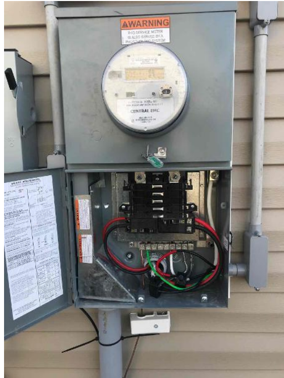
Electrical Information - Photo: Main Service Panel
