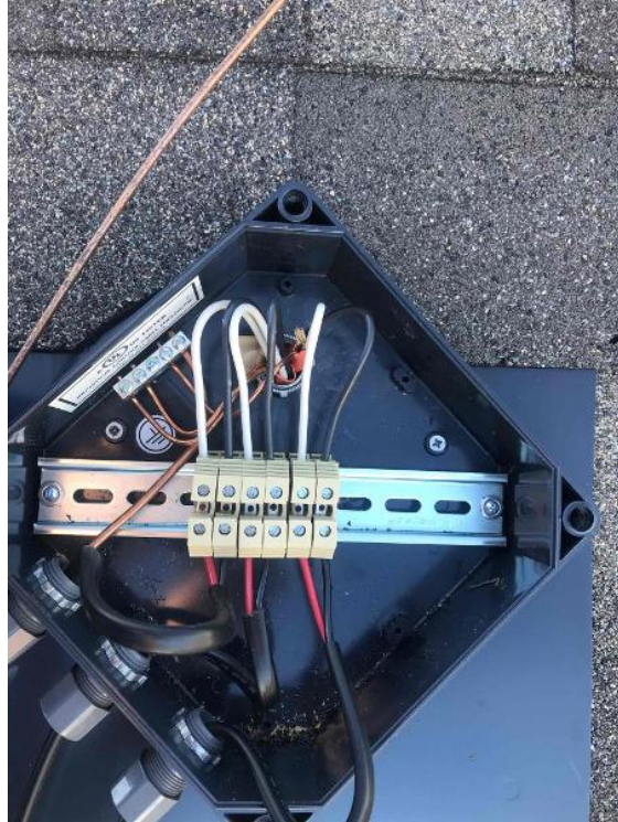
Roof/Array Information - Photo: Junction Box Location
