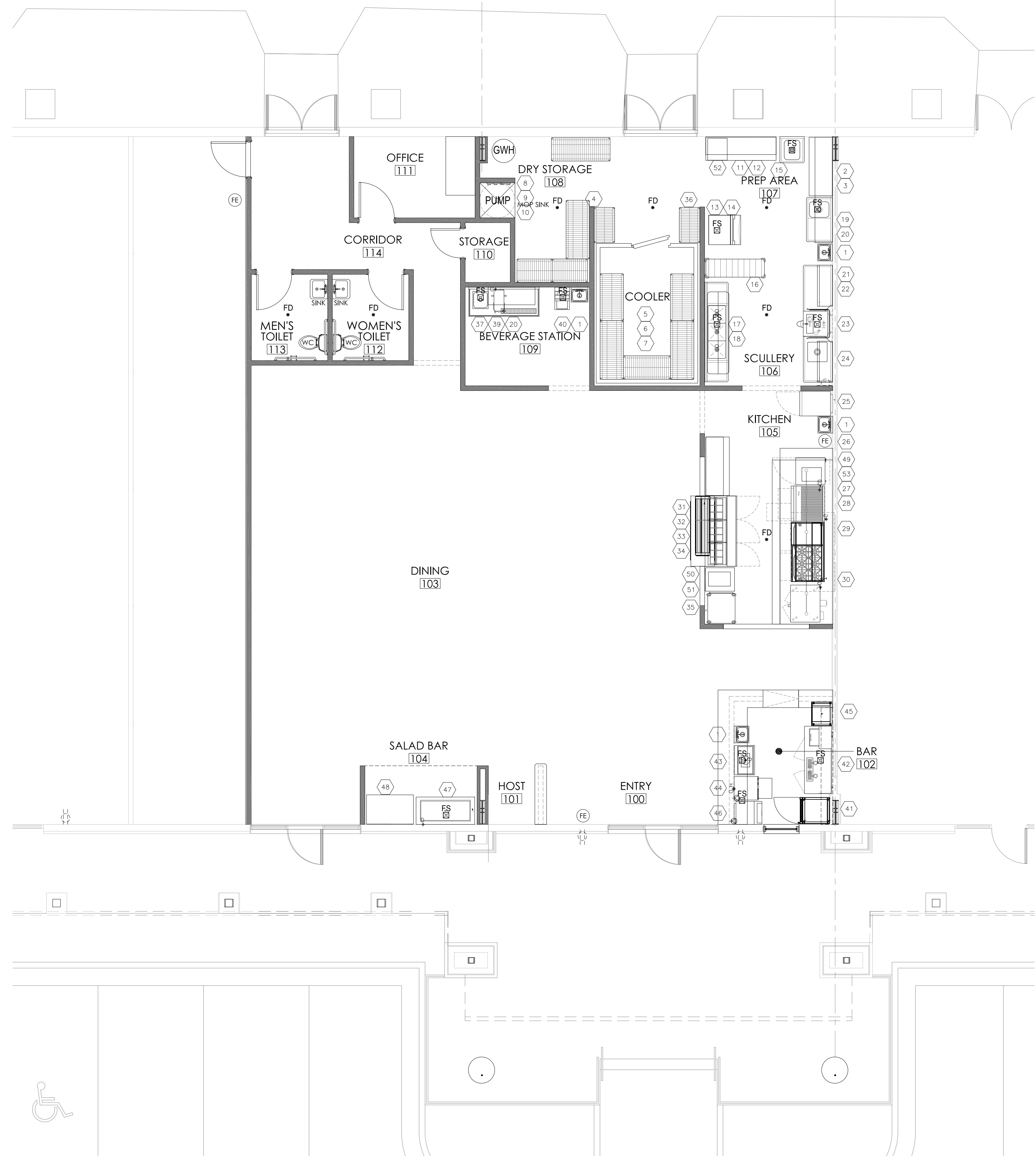
2 FOOD SERVICE PLAN SCALE: 3/16"=1'-0"
