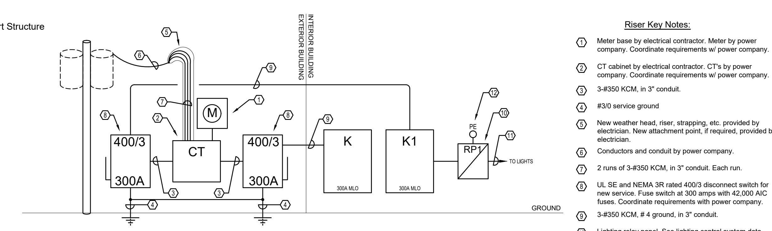
4 Electrical Riser Diagram Scale: None
