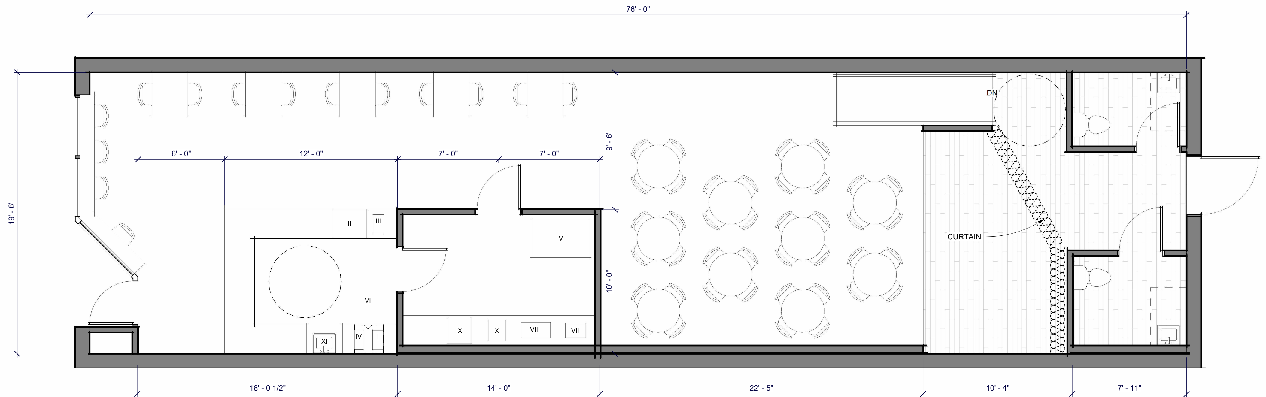
FLOOR PLAN - OPTION A 1 1/4" = 1'-0"
