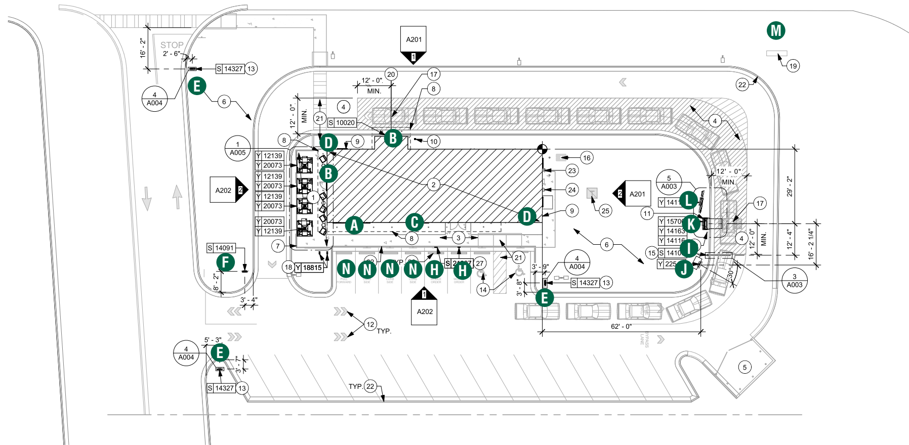
1 1ST FLOOR - SITE PLAN
