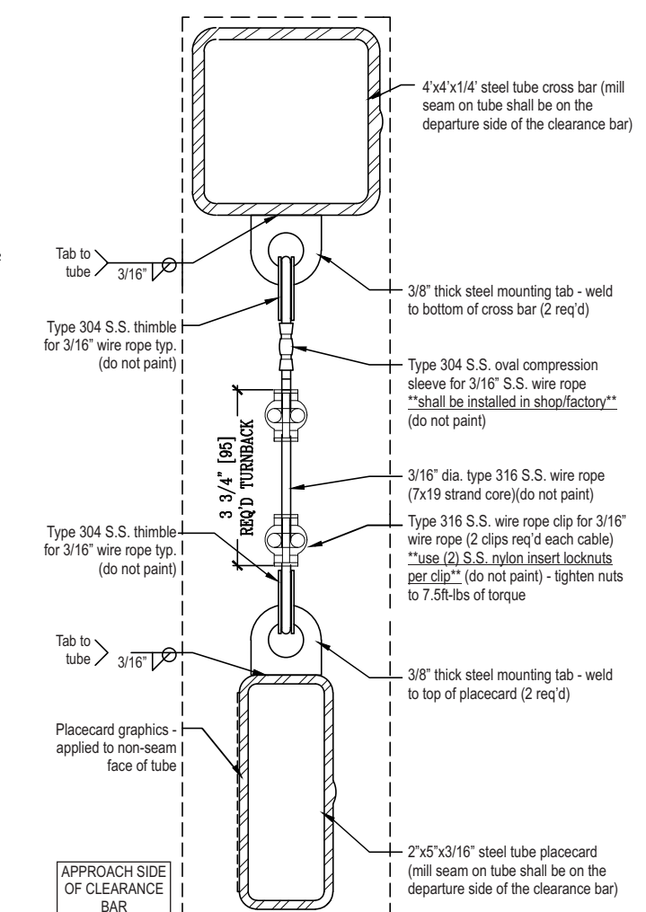
End Section View
