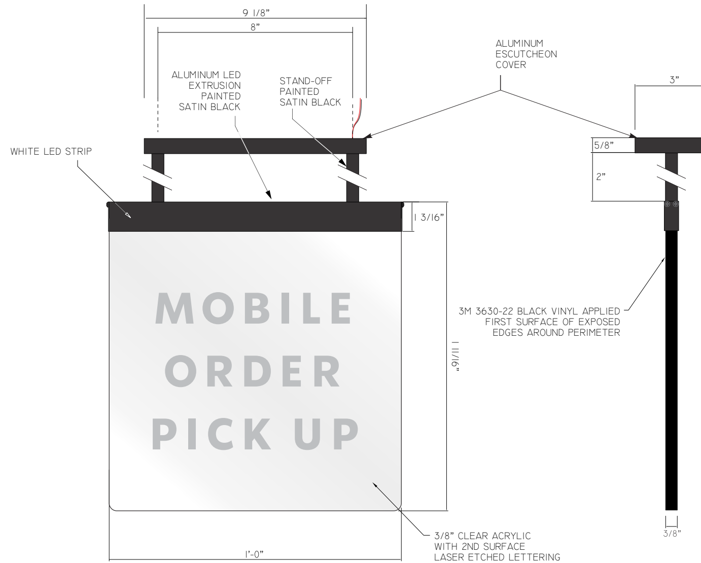
FRONT VIEW
