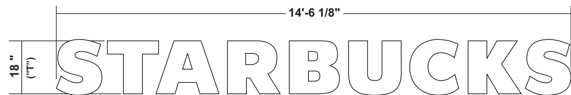
1 Front View Scale: 3/8" = 1' (11x17 Paper)
