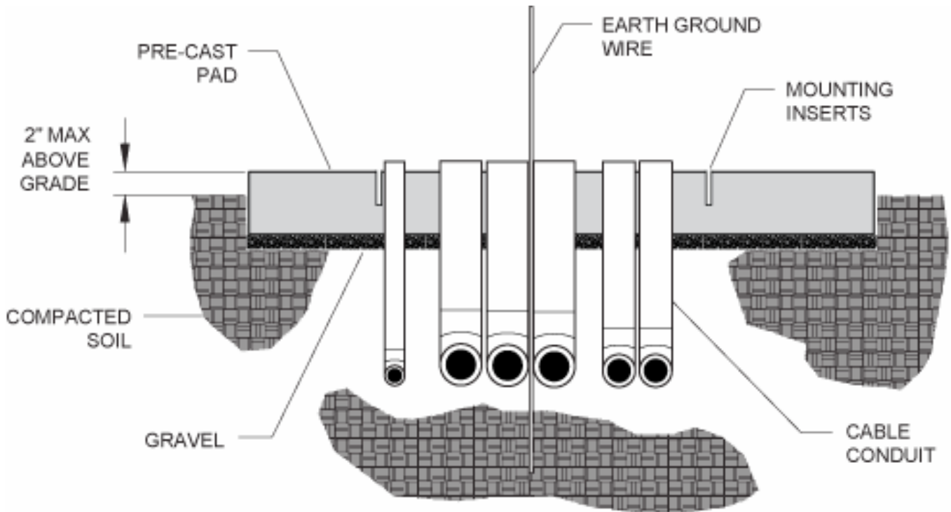
Pad Cross-Section
