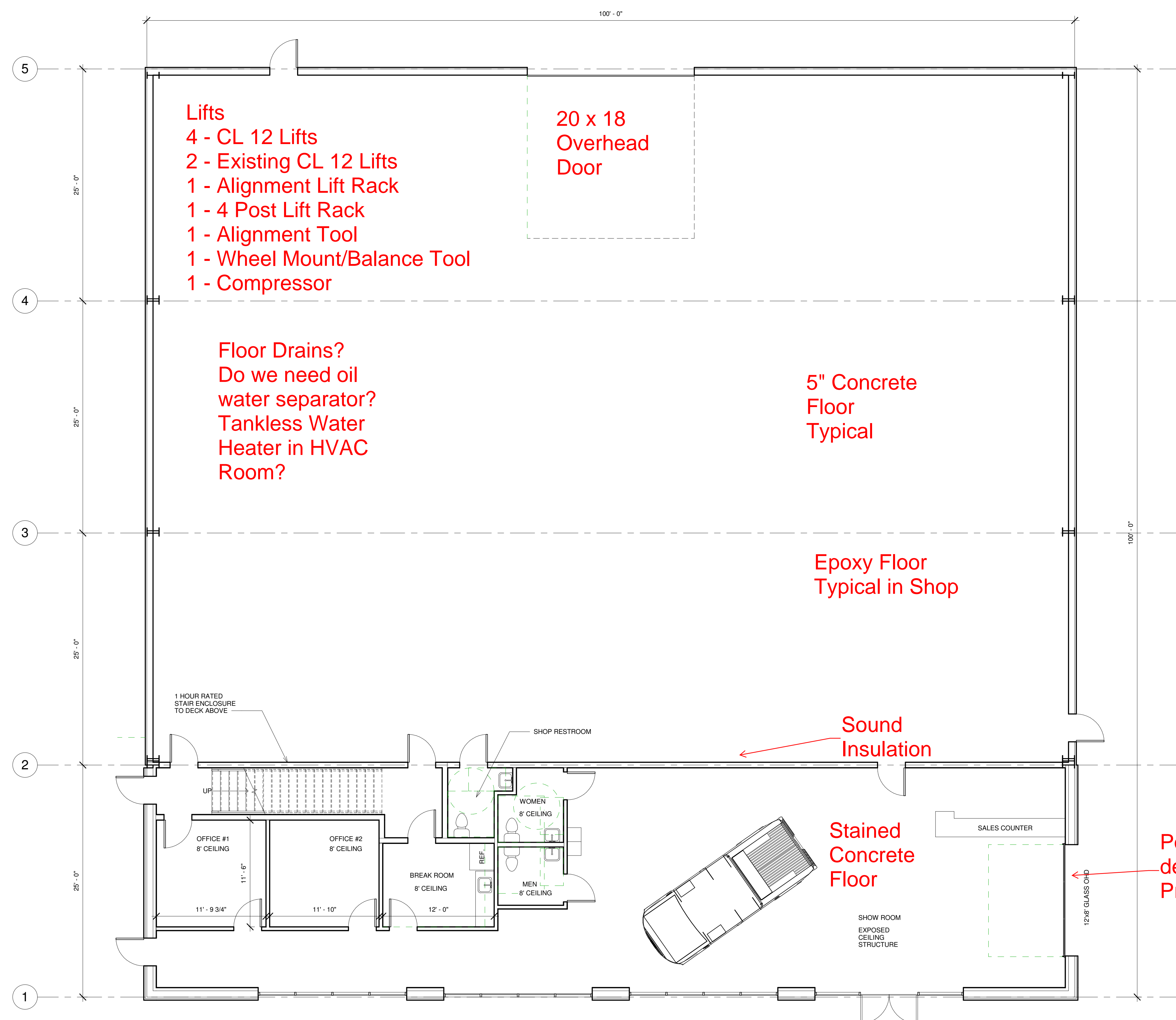
1 FIRST FLOOR PLAN 3/16" = 1'-0"
