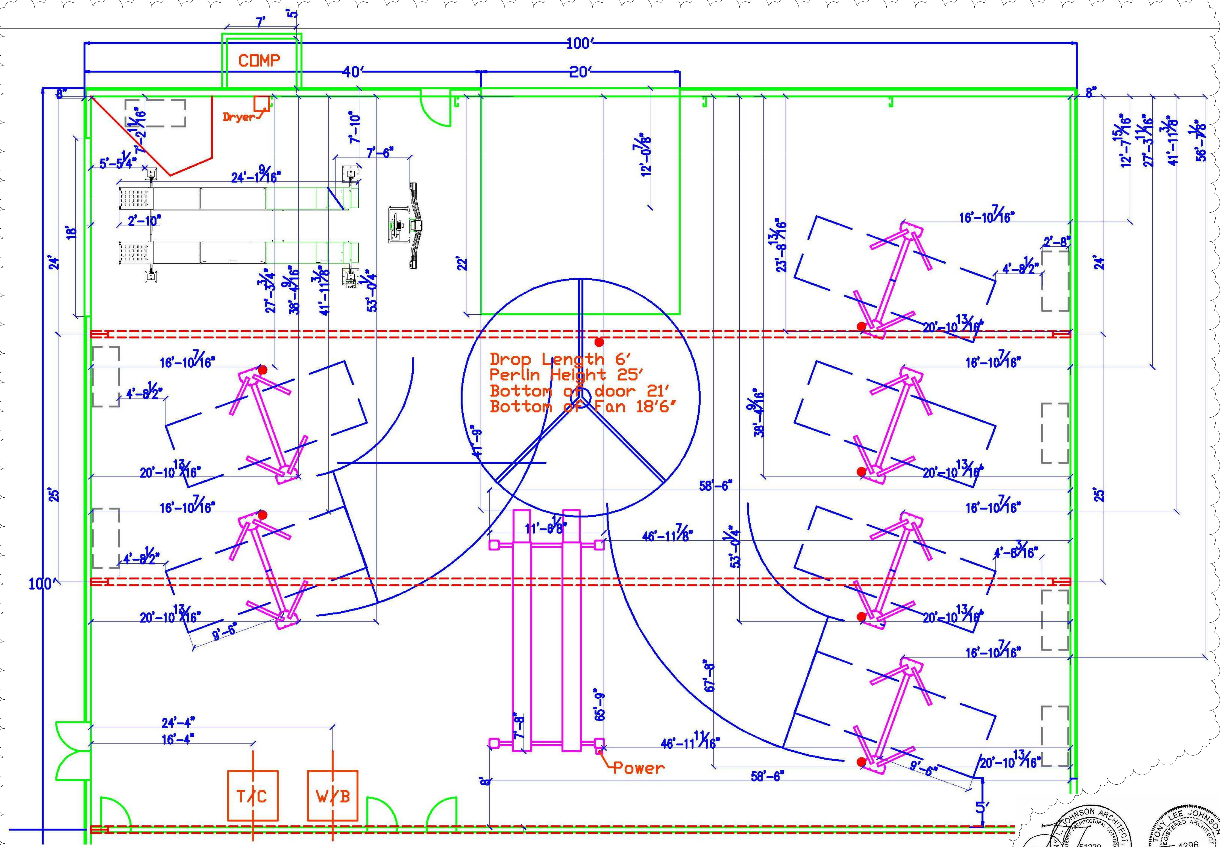
SHOP EQUIPMENT LAYOUT 1/4"=1'-0"
