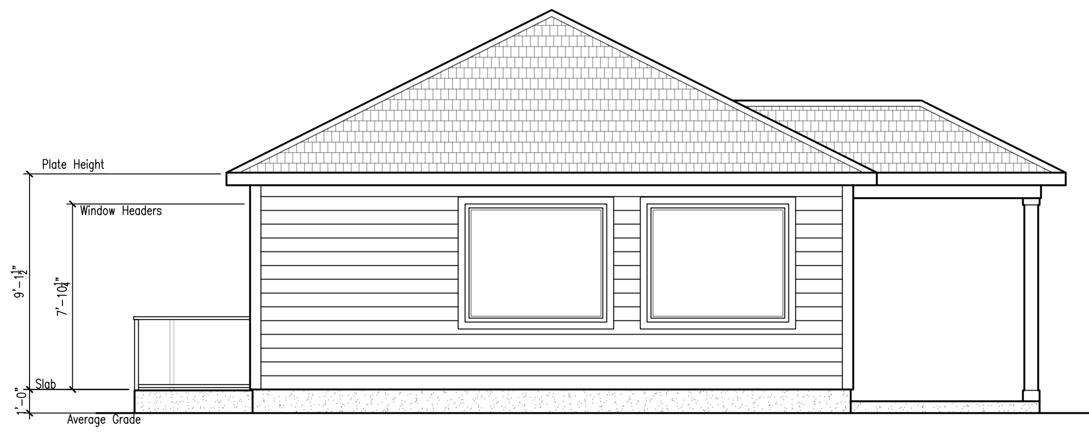
Front Elevation
