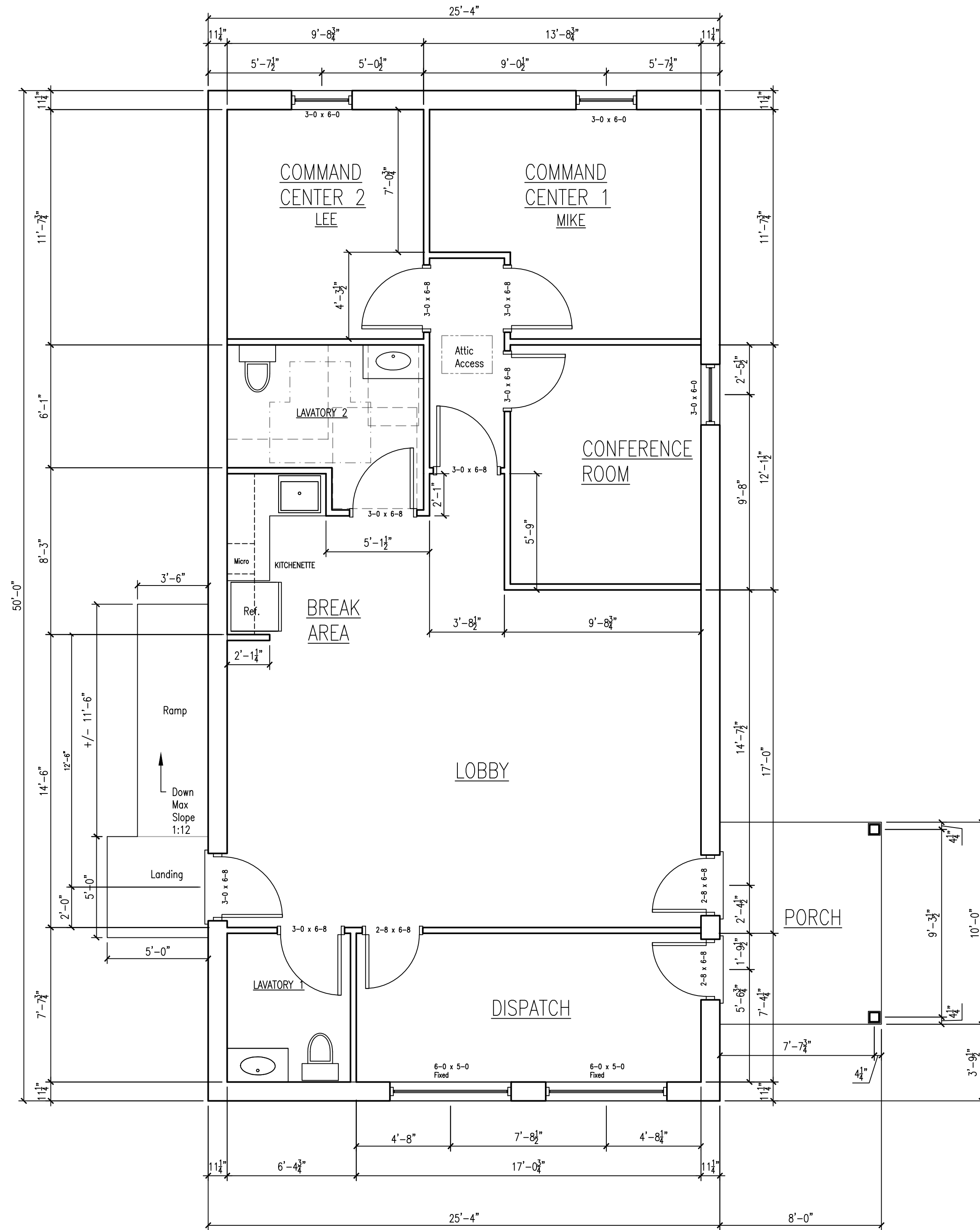
Floor Plan
