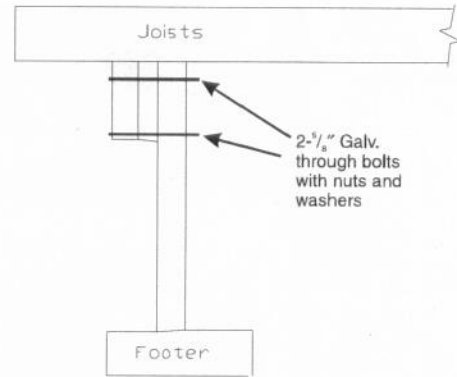
SIDE MOUNT DROPPED GIRDER FIGURE AM105.1
