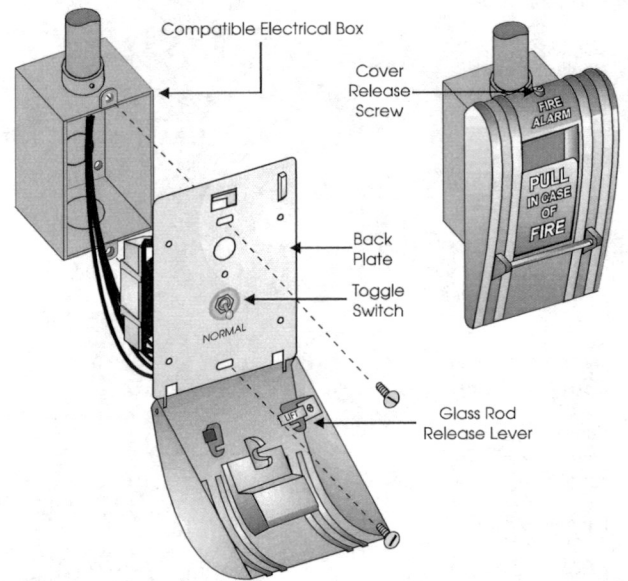
Figure 2. SIGA-270, SIGC-270F, SIGC-270B installation
