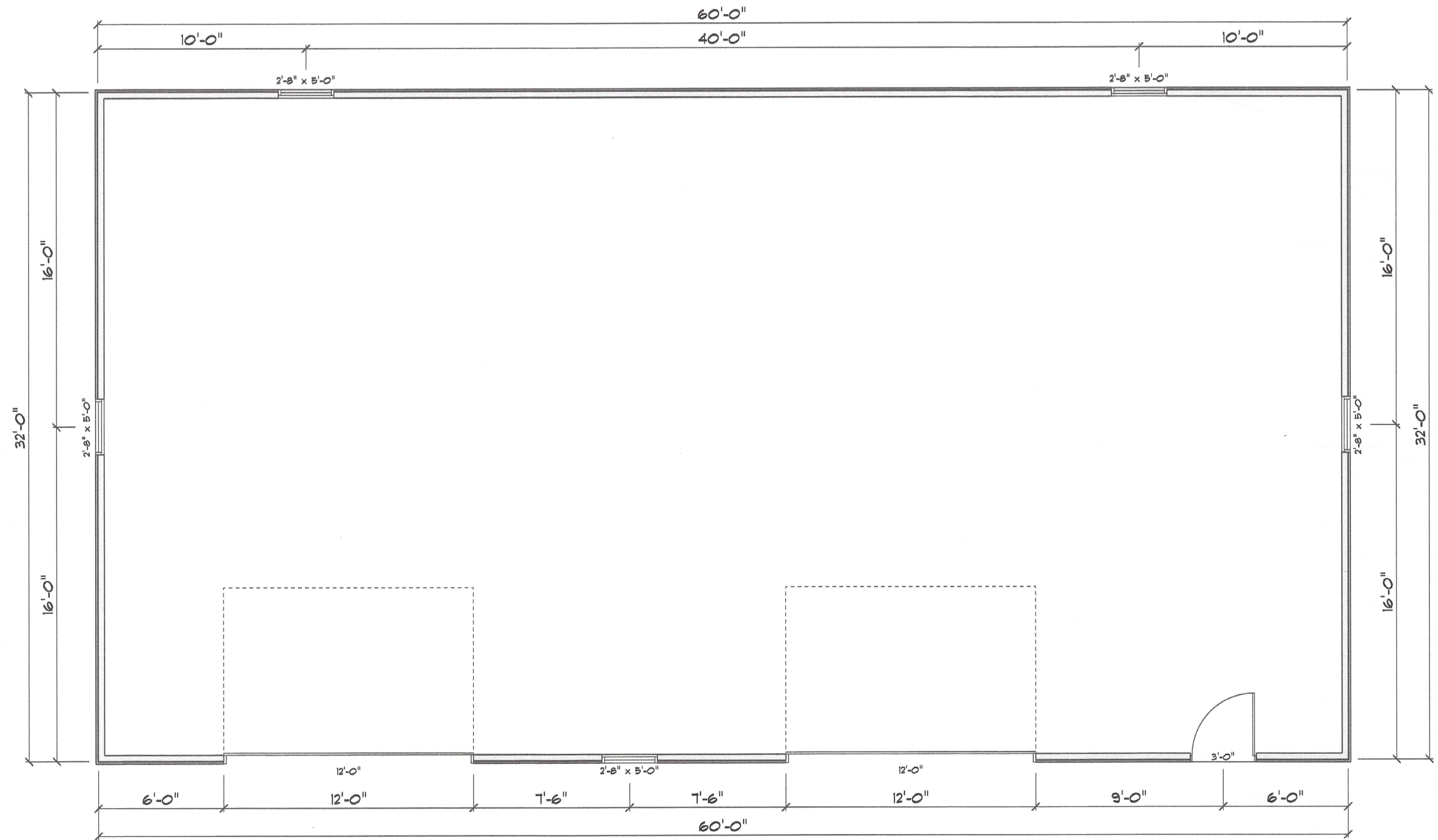
FLOOR PLAN SCALE: 1" = 1/4"
