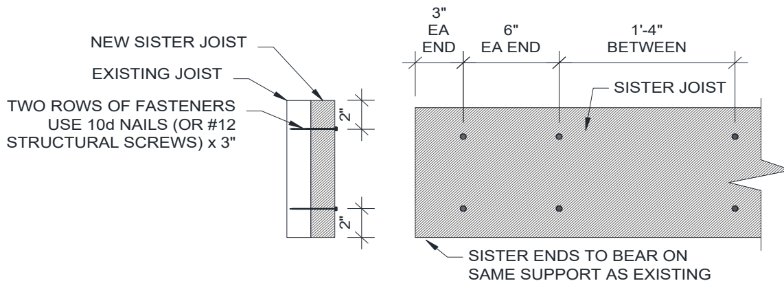
JOIST SISTER DETAIL
