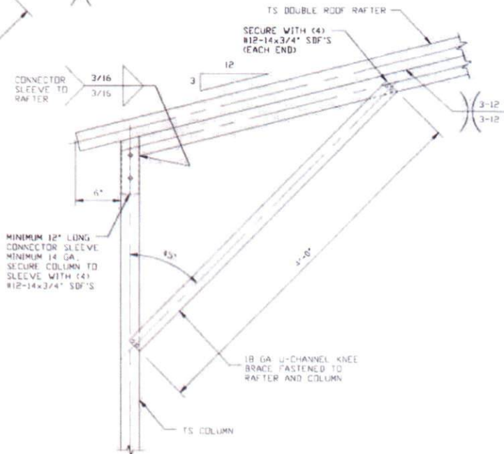
1B BOX EAVE RAFTER COLUMN CONNECTION DETAIL FOR HEIGHTS ≤ 12'-0" SCALE: NTS
