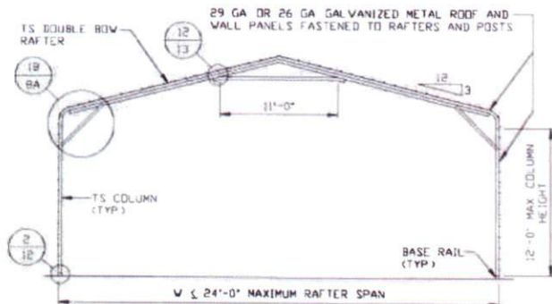
TYPICAL RAFTER/COLUMN END FRAME SECTION SCALE: NTS
