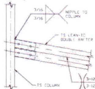
DOUBLE TUBE LEAN-TO RAFTER TO RAFTER COLUMN CONNECTION DETAIL
