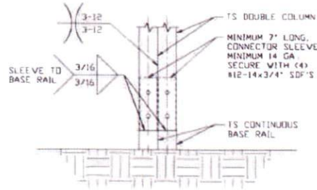
2A COLUMN/BASE RAIL CONNECTION DETAIL SCALE: NTS
