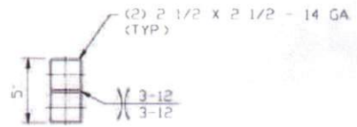
HEADER DETAIL FOR SIDE WALL DOOR OPENINGS < 11'-0"
