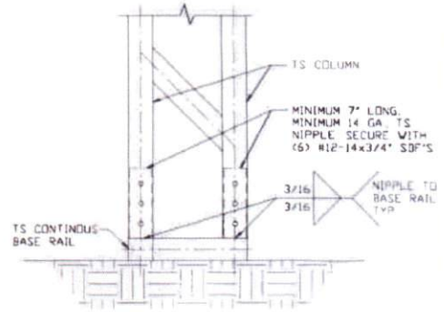
2B COLUMN/BASE RAIL CONNECTION DETAIL
