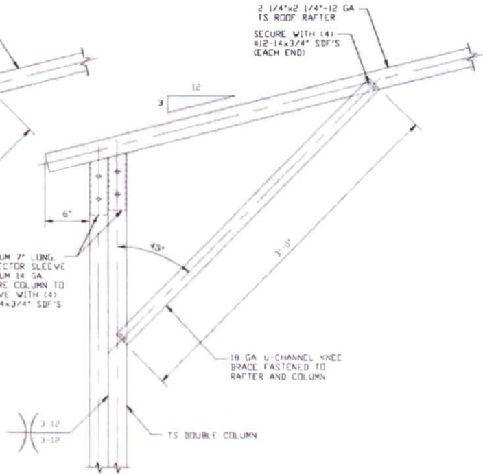
1D BOX EAVE RAFTER COLUMN CONNECTION DETAIL FOR HEIGHTS 12'-0" < TO ≤ 16'-0" SCALE: NTS
