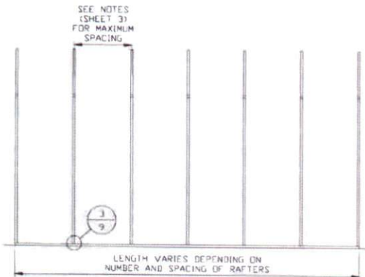
TYPICAL RAFTER/COLUMN SIDE FRAMING SECTION SCALE: NTS
