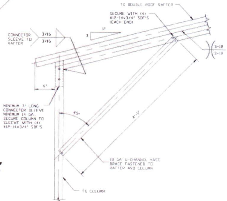
BOX EAVE RAFTER COLUMN CONNECTION DETAIL FOR HEIGHTS ≤ 12'-0" SCALE: NTS
