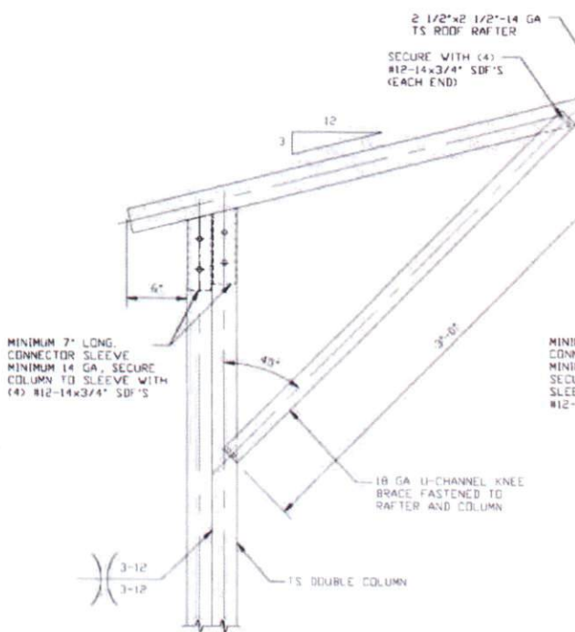
1C BOX EAVE RAFTER COLUMN CONNECTION DETAIL FOR HEIGHTS 12'-0" < TO ≤ 16'-0" SCALE: NTS
