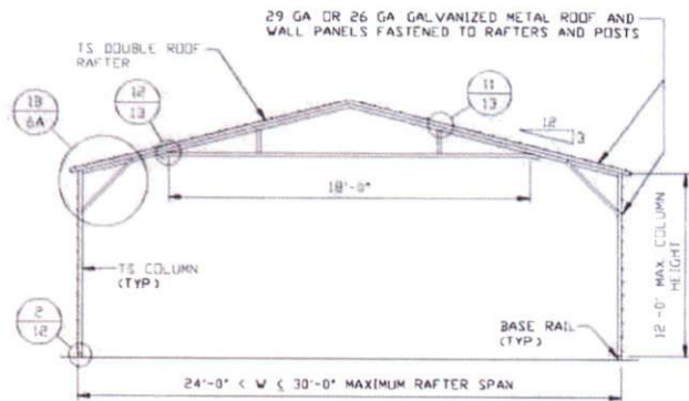
TYPICAL RAFTER/COLUMN END FRAME SECTION SCALE: NTS
