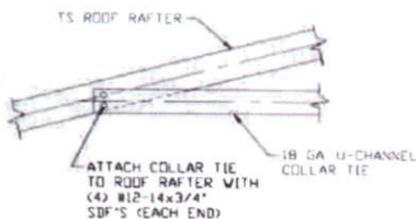
12B COLLAR TIE CONNECTION DETAIL SCALE: NTS
