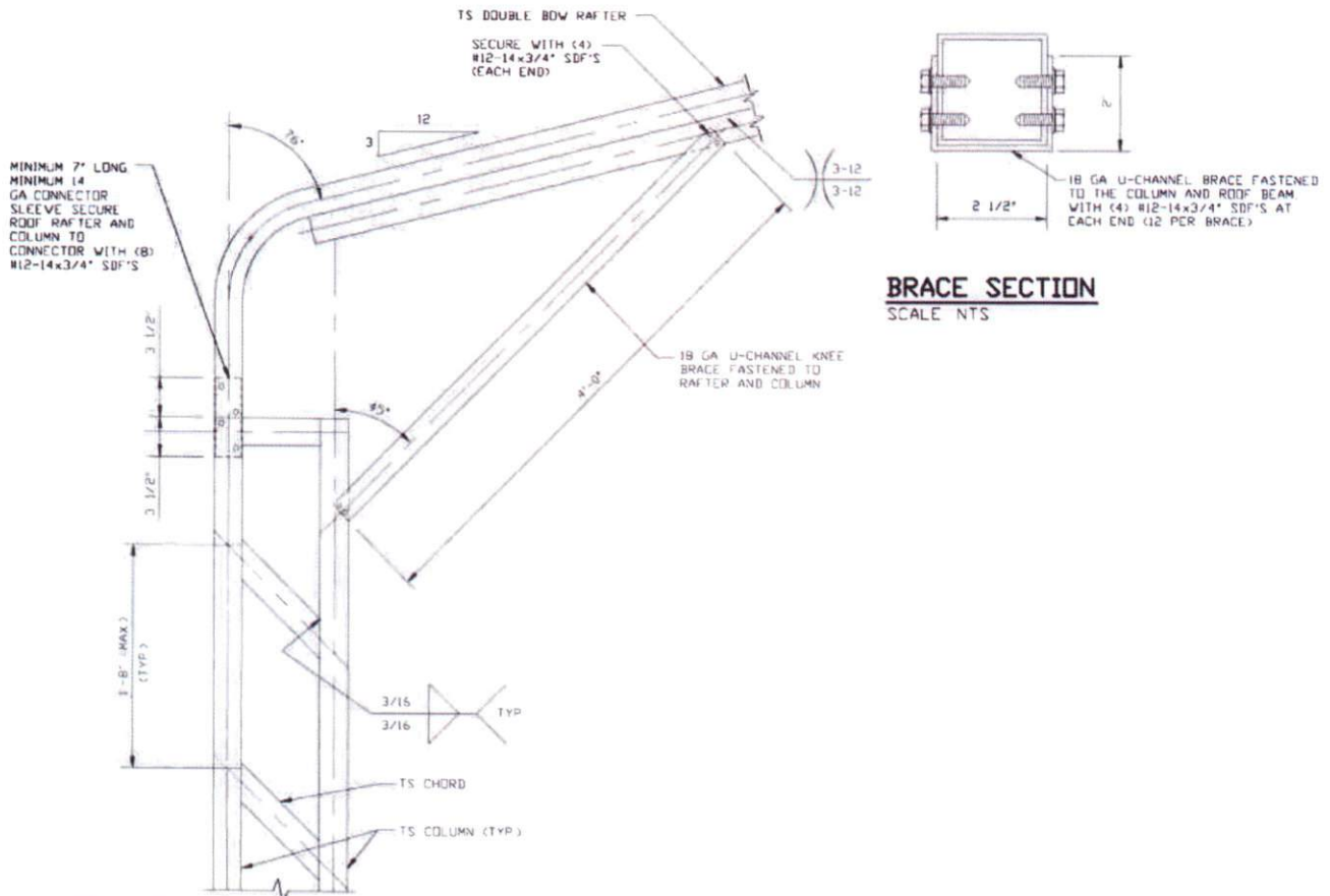
BOW EAVE RAFTER COLUMN CONNECTION DETAIL FOR HEIGHTS 16'-0" < TO ≤ 20'-0"
