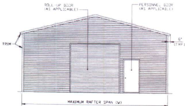
TYPICAL END ELEVATION SCALE: NTS
