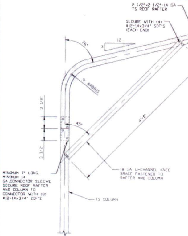
1E BOW EAVE RAFTER COLUMN CONNECTION DETAIL FOR HEIGHTS ≤ 12'-0" SCALE: NTS
