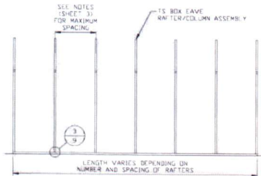
TYPICAL RAFTER/COLUMN SIDE FRAMING SECTION SCALE: NTS
