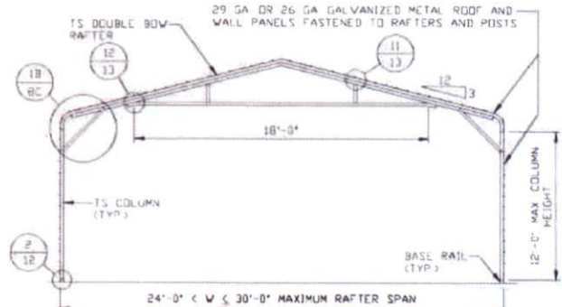
TYPICAL RAFTER/COLUMN SIDE FRAMING SECTION SCALE: NTS
