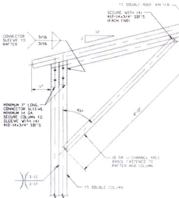
1A BOX EAVE RAFTER COLUMN CONNECTION DETAIL FOR HEIGHTS 12'-0" < TO ≤ 16'-0" SCALE: NTS
