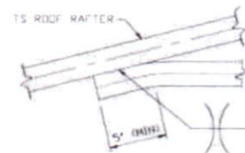
12A COLLAR TIE CONNECTION DETAIL SCALE: NTS
