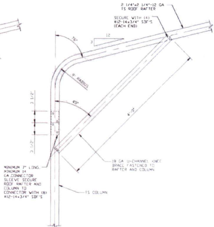
1F BOW EAVE RAFTER COLUMN CONNECTION DETAIL FOR HEIGHTS ≤ 12'-0" SCALE: NTS
