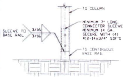
2 COLUMN/BASE RAIL CONNECTION DETAIL SCALE: NTS
