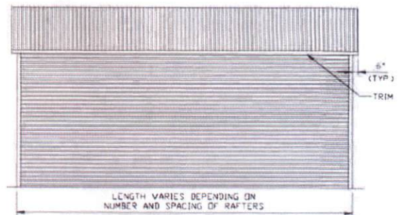
TYPICAL SIDE ELEVATION-VERTICAL ROOF OPTION SCALE: NTS
