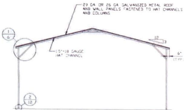
TYPICAL SECTION-VERTICAL ROOF SCALE: NTS
