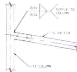
LEAN-TO RAFTER TO RAFTER COLUMN CONNECTION DETAIL
