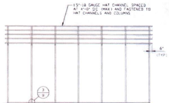
TYPICAL FRAMING SECTION-VERTICAL ROOF OPTION SCALE: NTS
