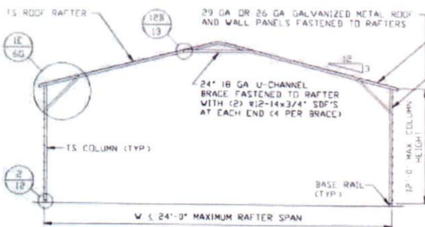
TYPICAL RAFTER/COLUMN END FRAME SECTION SCALE: NTS
