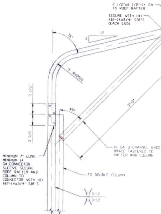
1C BOW EAVE RAFTER COLUMN CONNECTION DETAIL FOR HEIGHTS 12'-0" < TO ≤ 16'-0" SCALE: NTS
