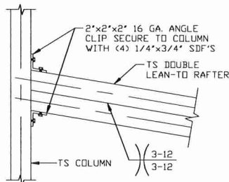
LEAN-TO RAFTER TO RAFTER POST CONNECTION DETAIL FOR WIDTHS
