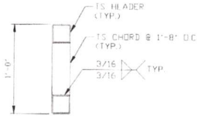
HEADER DETAIL FOR SIDE WALL DOOR OPENINGS 14'-0'' < \text{LENGTH} \leq 16'-0'' SCALE: NTS
