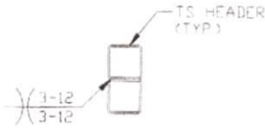
HEADER DETAIL FOR SIDE WALL DOOR OPENINGS 8'-0'' < \text{LENGTH} \leq 14'-0'' SCALE: NTS
