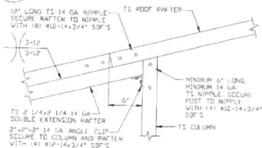
SIDE EXTENSION RAFTER COLUMN DETAIL FOR SPANS 12'-0" < TO < 16'-0"
