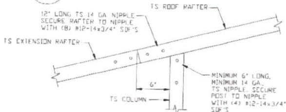
SIDE EXTENSION RAFTER COLUMN DETAIL FOR SPANS ≤ 12'-0"
