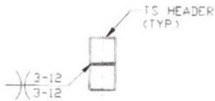
HEADER DETAIL FOR SIDE WALL DOOR OPENINGS 13'-0'' < \text{LENGTH} \leq 16'-0'' SCALE: NTS
