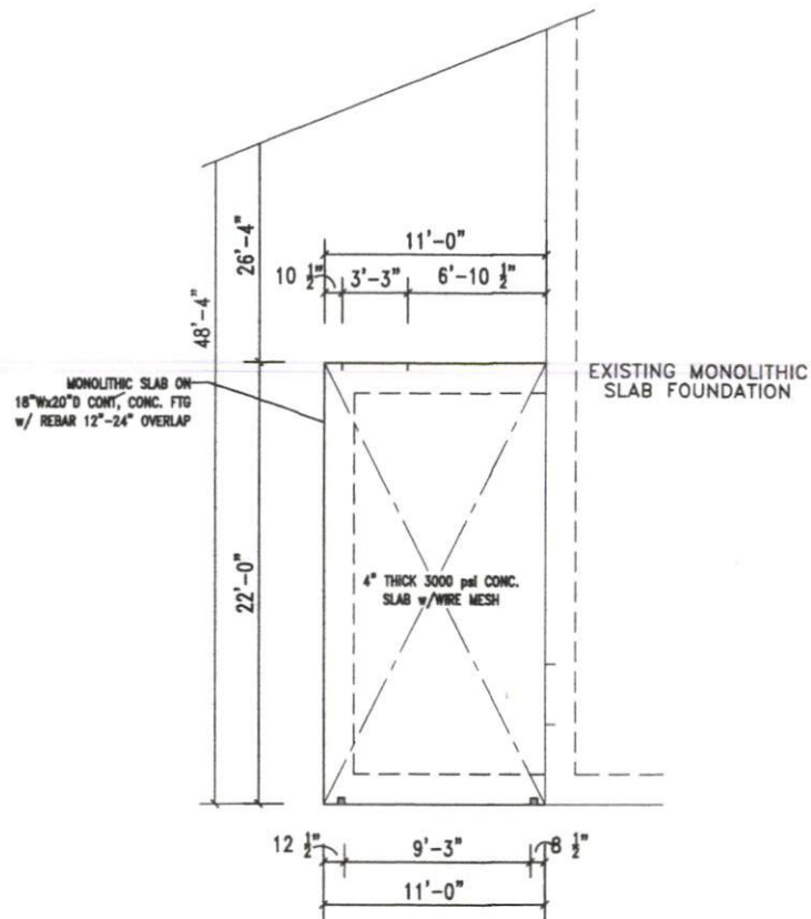
FOUNDATION SCALE:.....1/8"=1'
