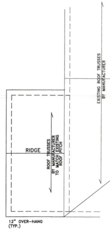
ROOF FRAMING SCALE:.....1/8"=1'
