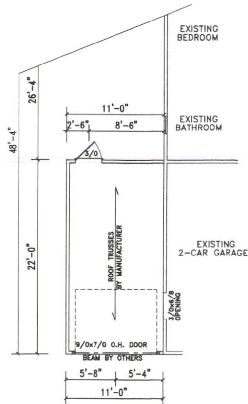
FLOOR PLAN DETAIL SCALE:.....1/8"=1' NOTE: 8'-0" CLG. HGT.
