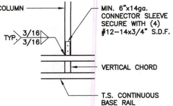
2 S13 LACED HEADER / COLUMN CONNECTION DETAIL
