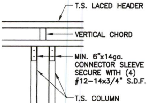
3 S13 LACED HEADER / COLUMN CONNECTION DETAIL
