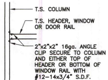
HEADER / GIRT TO COLUMN CONNECTION DETAIL
