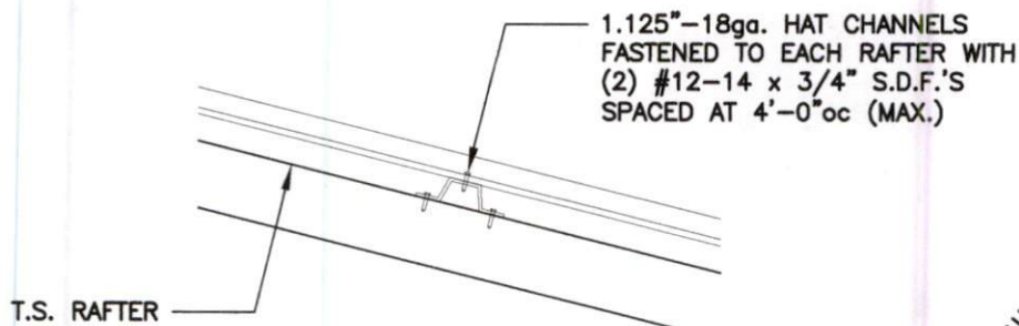
(TYPICAL) ROOF PANEL ATTACHMENT
