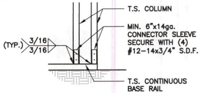
DOOR COLUMN / BASE RAIL CONNECTION DETAIL
