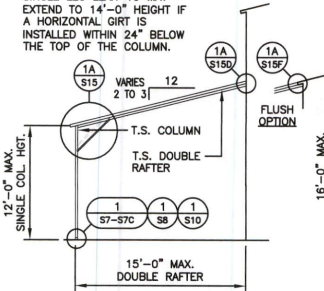
DOUBLE RAFTER / SINGLE COLUMN LEAN-TO FRAMING SECTION
