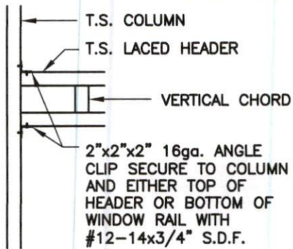
1 S13 COLUMN / LACED HEADER CONNECTION DETAIL
