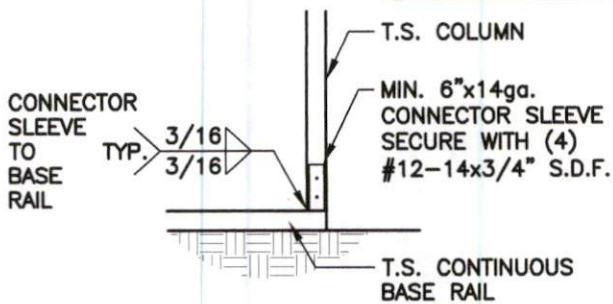
DOOR COLUMN / BASE RAIL CONNECTION DETAIL
