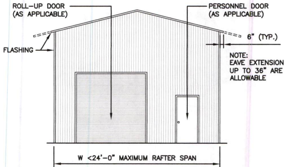
TYPICAL END ELEVATION - VERTICAL ROOF / SIDING
