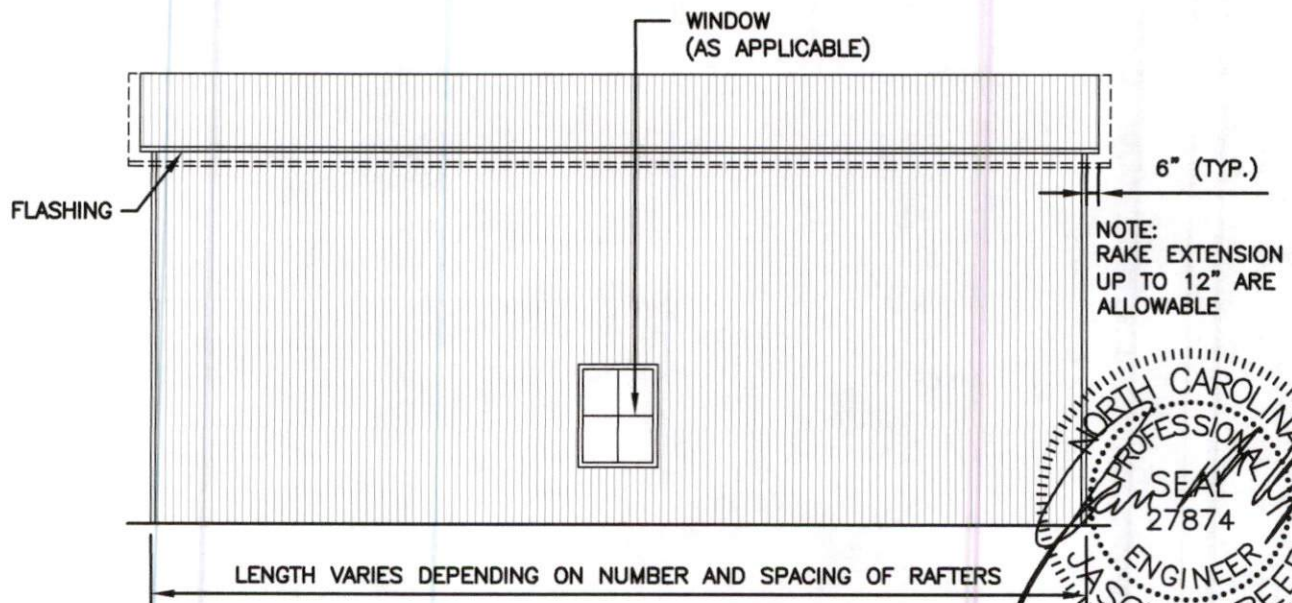
TYPICAL SIDE ELEVATION - VERTICAL ROOF / SIDING
