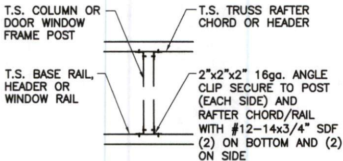
COLUMN TO RAIL CONNECTION DETAIL
