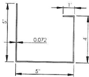
STRUCTURAL GUTTER
