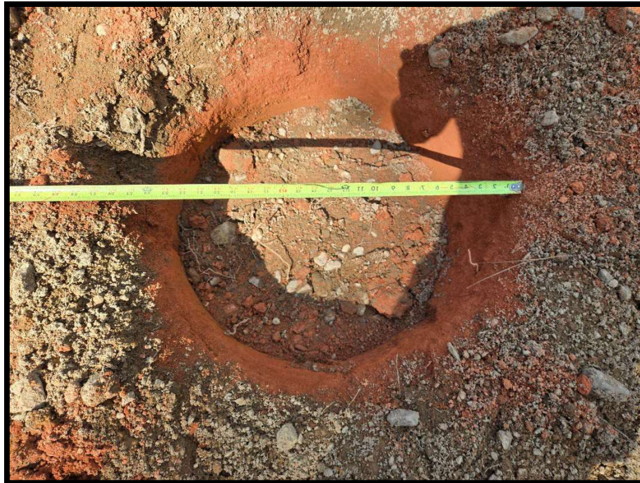
(Width and Depth of Pier Foundation)
