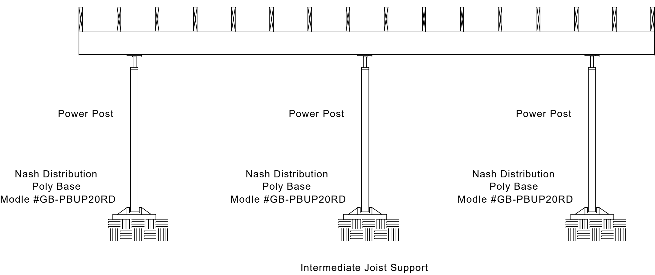
Maximum Girder Spans for Power Post with 18" Poly Base
