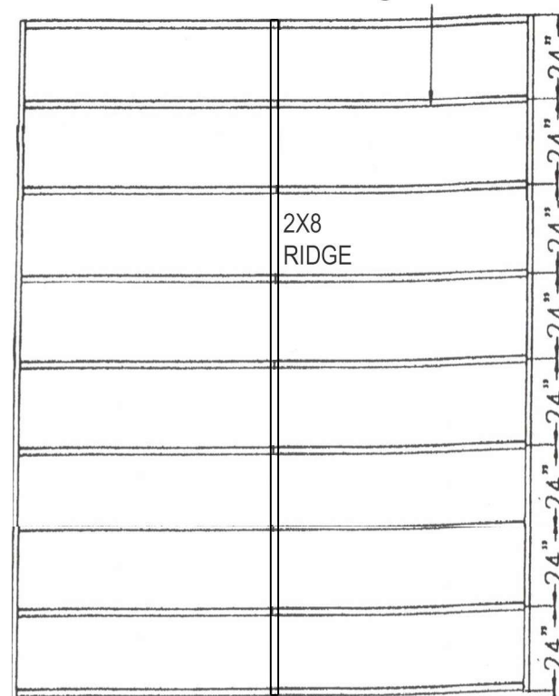
ROOF FRAMING
