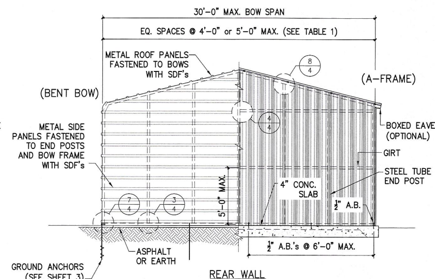
REAR WALL
