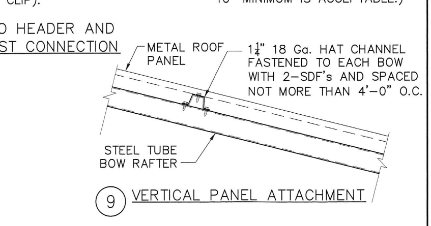
10 VERTICAL PANEL ATTACHMENT
