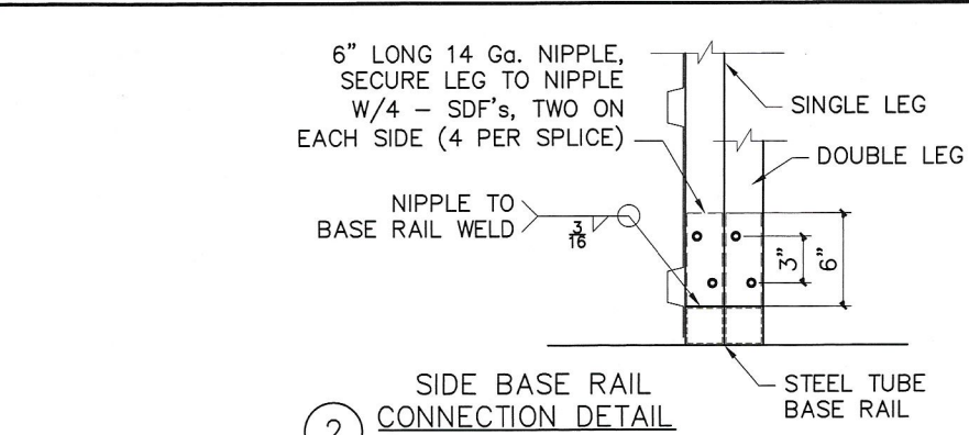
3 SIDE BASE RAIL CONNECTION DETAIL
