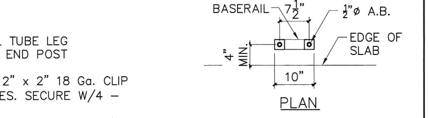
8 SECTION THROUGH ROLL-UP DOOR POST
