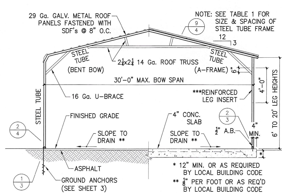
1 2 TYPICAL BOW SECTION
