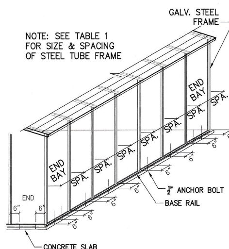
ANCHOR BOLTS
