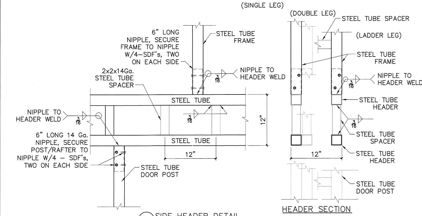
2 SIDE HEADER DETAIL (LADDER STYLE FOR 13' TO 20' OPENING)
