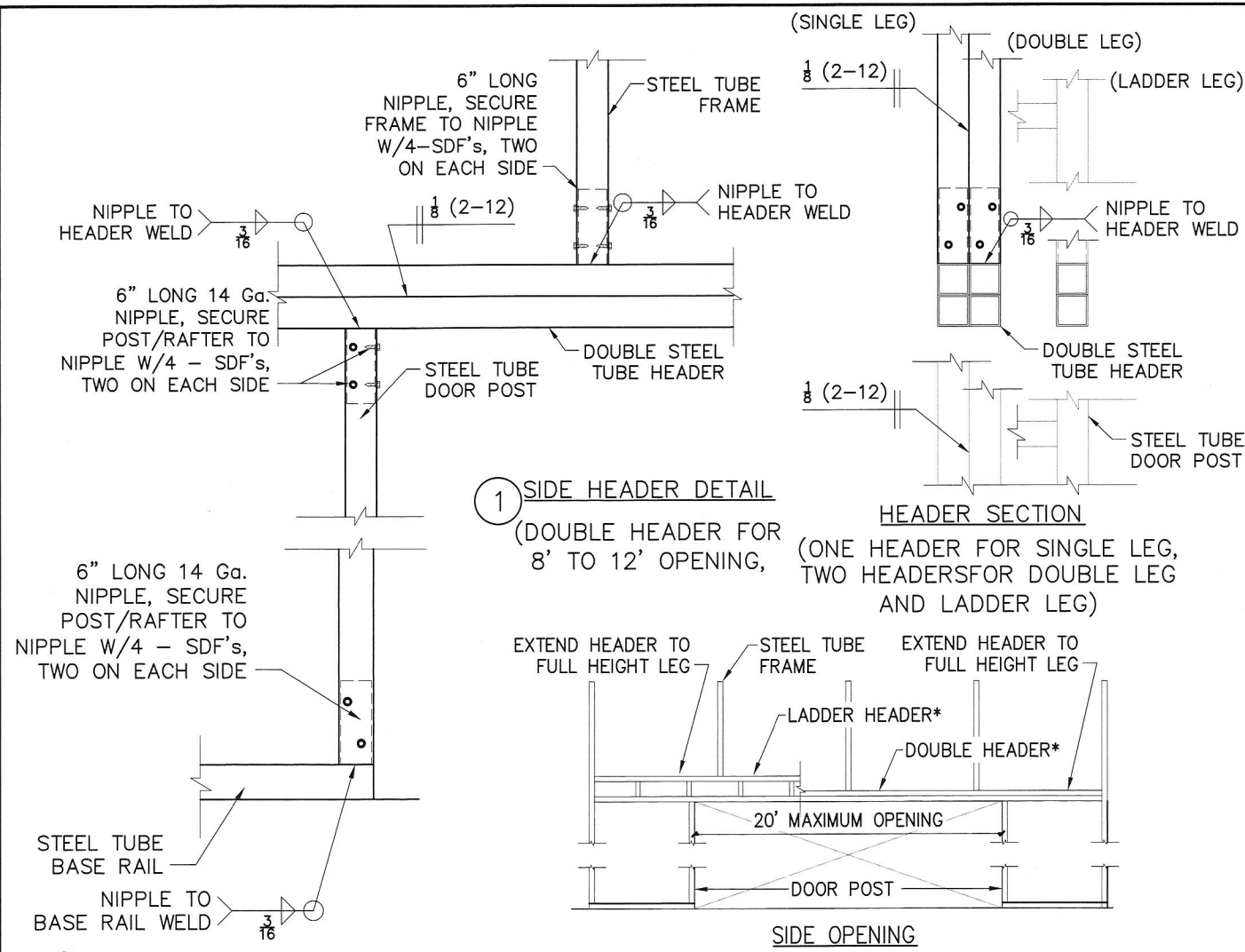
1 SIDE HEADER DETAIL (DOUBLE HEADER FOR 8' TO 12' OPENING, (ONE HEADER FOR SINGLE LEG, TWO HEADERS FOR DOUBLE LEG AND LADDER LEG)
