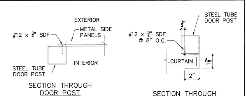
7 SECTION THROUGH DOOR POST
