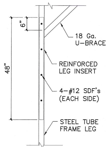
***REINFORCED LEG INSERT (LEG HEIGHTS 13' to 14')
