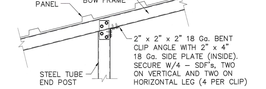
6 END POST TO BOW FRAME CONNECTION
