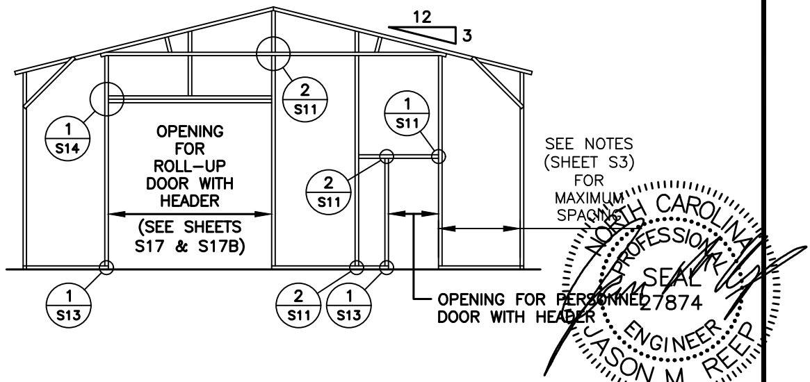
TYPICAL BOX EVE RAFTER END WALL OPENINGS FRAMING SECTION
