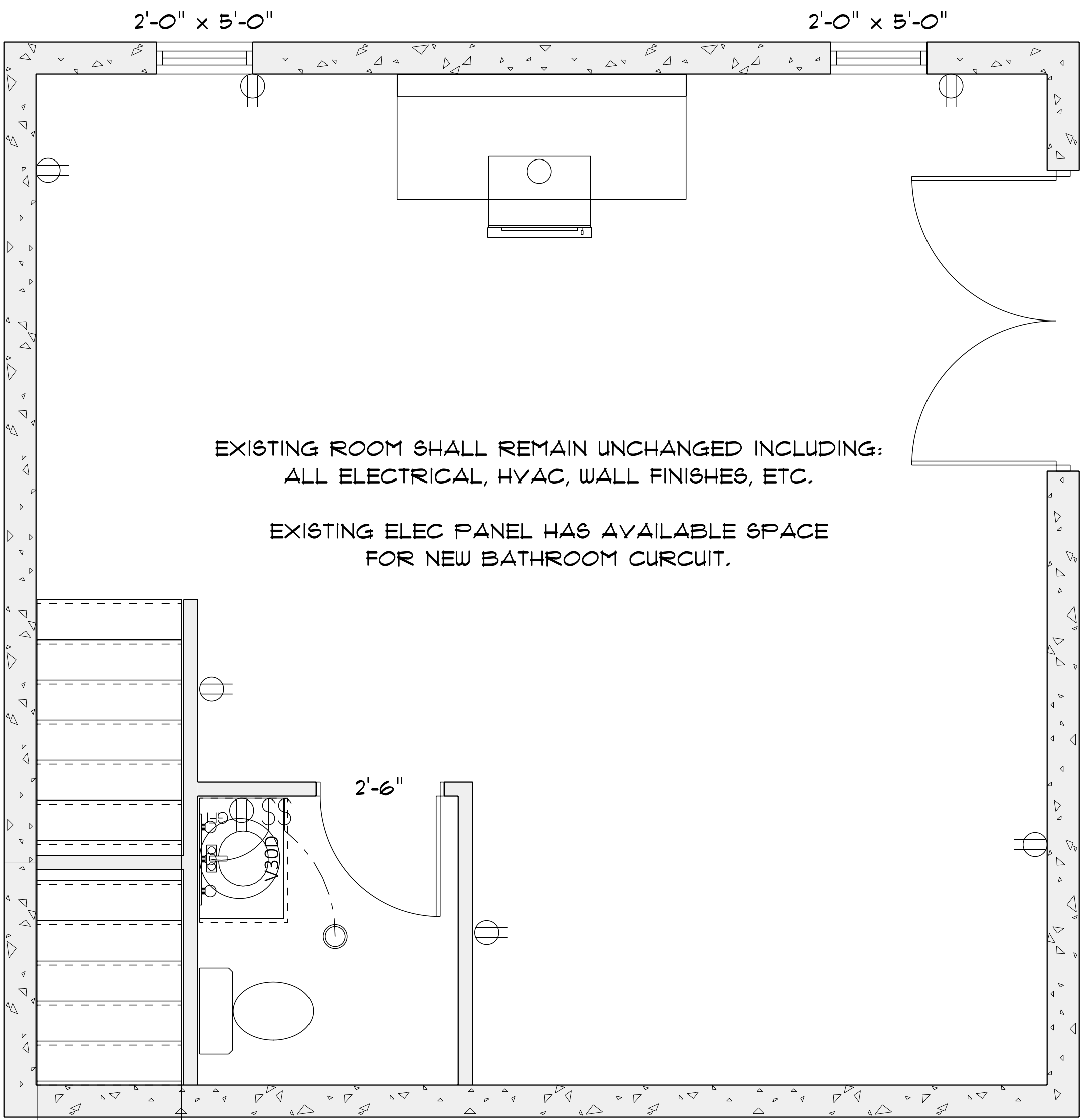
ELECTRICAL / LIGHTING SCALE: 1/2" = 1'-0"
