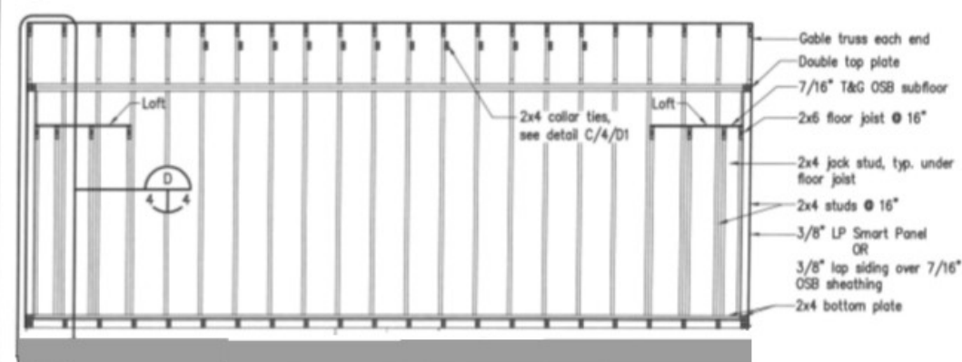
Wall Framing Elevation
