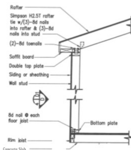
Wall Section
